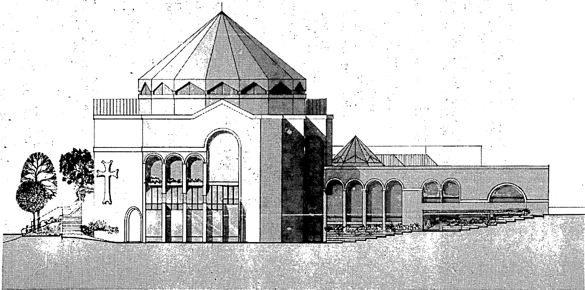
south elevation
