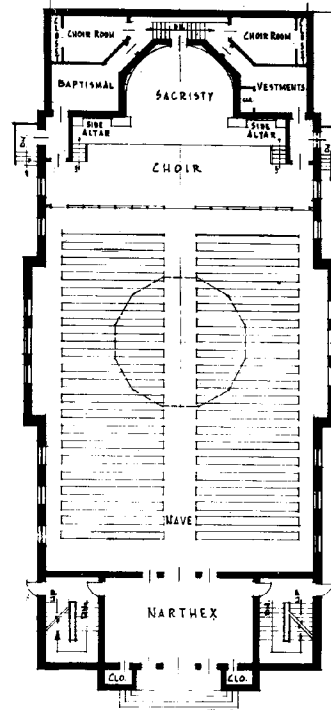
CHURCH PLAN FIRST FLOOR PLAN
