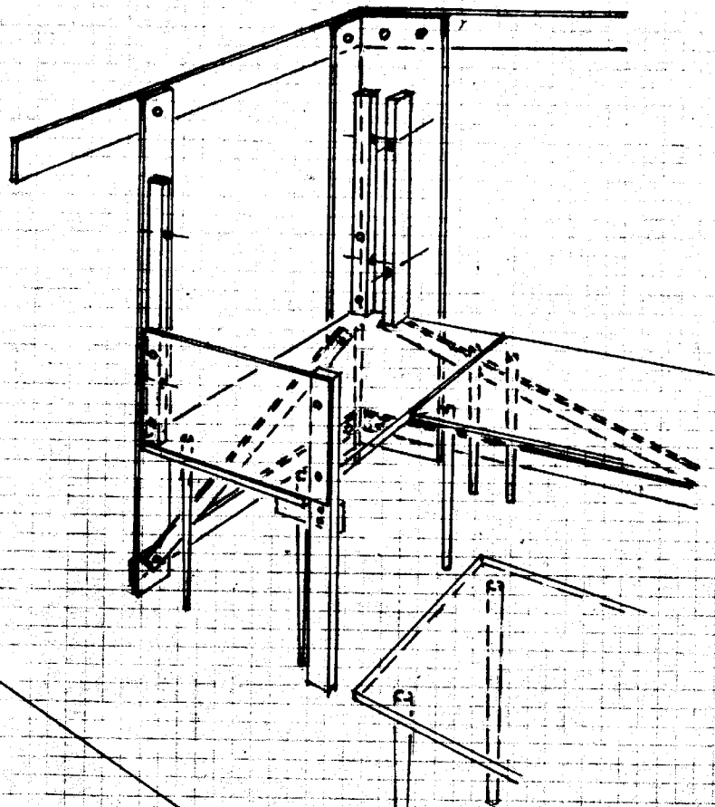
CORNER BOOTH CONSTRUCTION DETAILS
