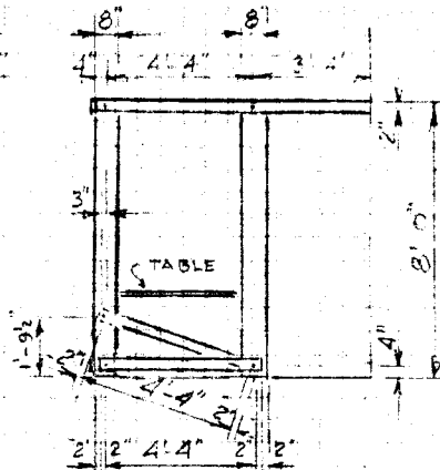
SIDE ELEVATION
