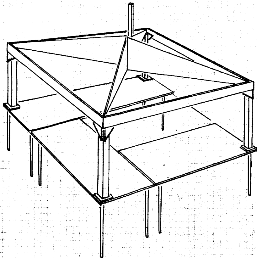
KIOSK CONSTRUCTION DETAILS
